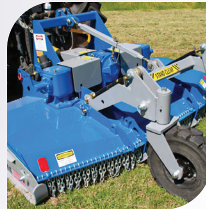
VHD Taper Back 3PL Twin Rotor General Slashers
